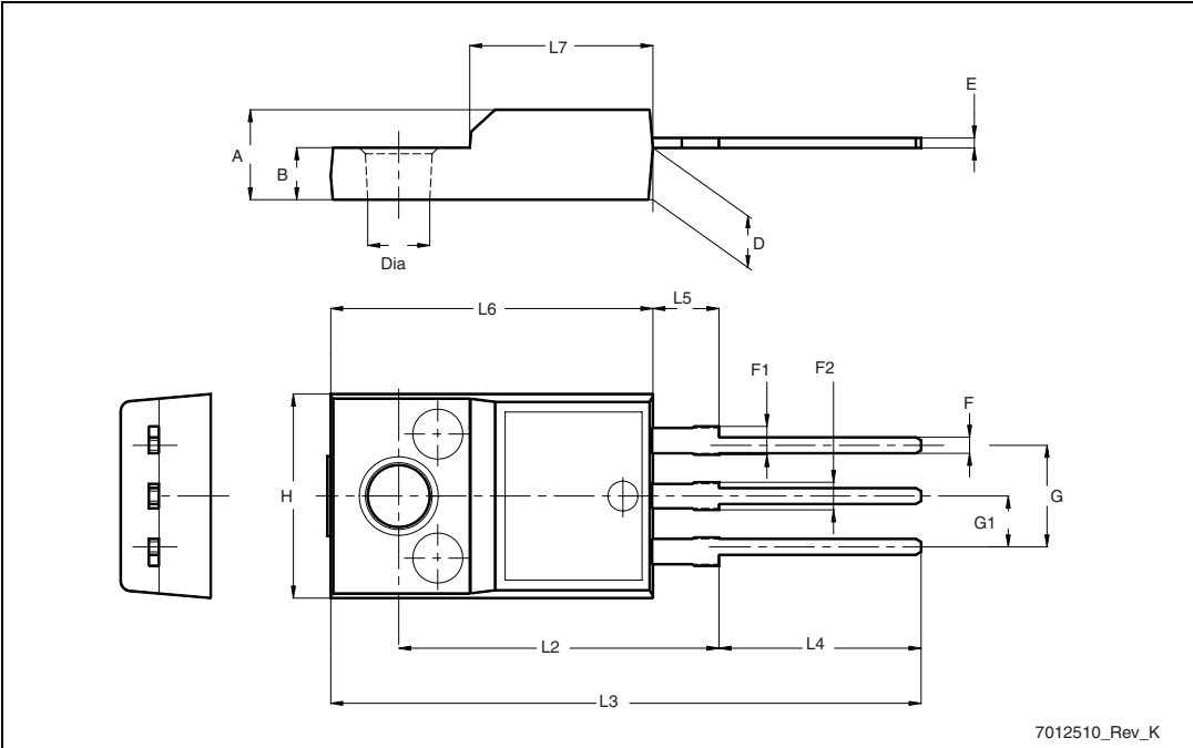
Figure 25. TO-220FP drawing
