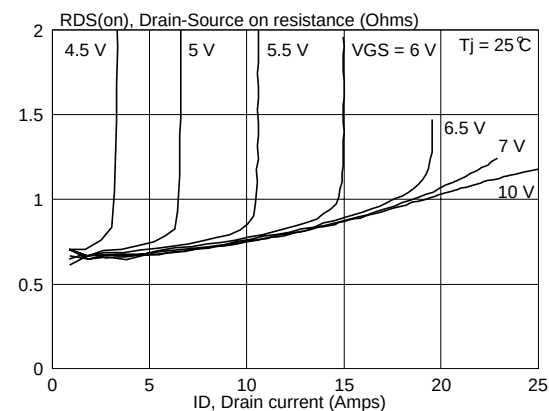
Fig.6. Typical on-state resistance. R_{DS(ON)} = f(I_D); \text{ parameter } V_{GS}
