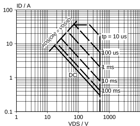
Fig.3. Safe operating area. T_{mb} = 25^\circ C I_D \text{ \& } I_{DM} = f(V_{DS}); I_{DM} \text{ single pulse; parameter } t_p
