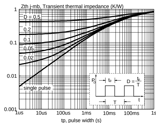
Fig.4. Transient thermal impedance. Z_{th\ j-mb} = f(t); \text{ parameter } D = t_p / T
